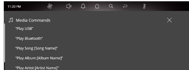
Figure 30 Voice Assistant Media Commands
