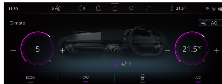
Figure 62 Climate Control
