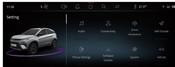
Figure 69 Settings
