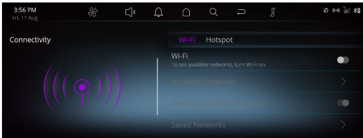
Figure 76 Wi-Fi
