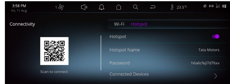
Figure 77 Hotspot
