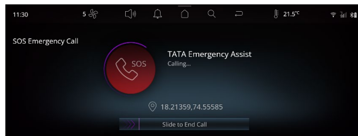
Figure 67 Emergency Call
