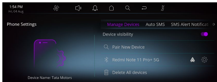
Figure 15 Manage Devices
