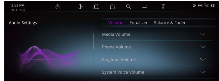
Figure 71 Audio Settings - 2
