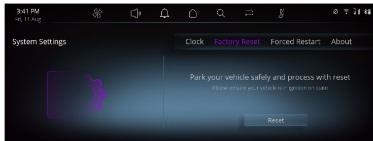
Figure 80 Factory Reset
