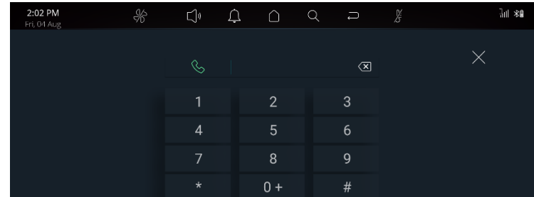
Figure 19 Dial Pad
