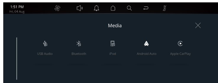
Figure 12 Media Screen
