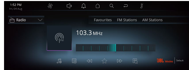
Figure 13 Radio Screen
