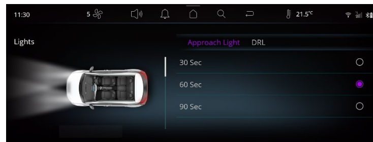
Figure 64 Approach lamp
