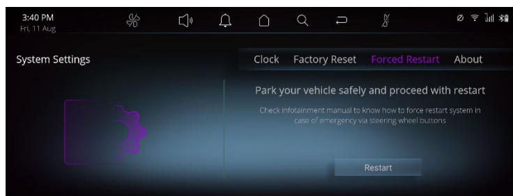
Figure 81 Force Restart
