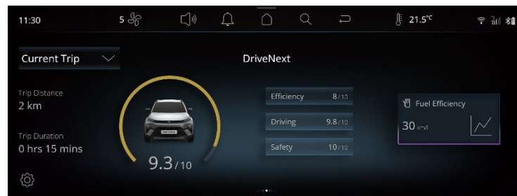
Figure 37 DriveNext Insights
