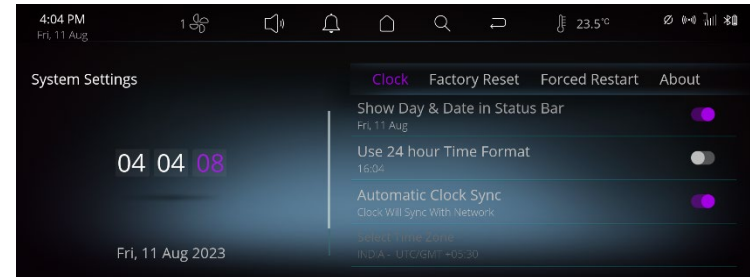
Figure 79 Setting Time
