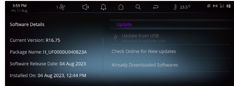
Figure 78 Software Details
