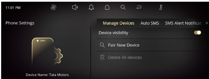
Figure 76 Phone Settings Screen
